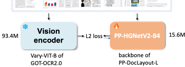
Figure 2. Knowledge Distillation Framework for the backbone of PP-DocLayout-L
